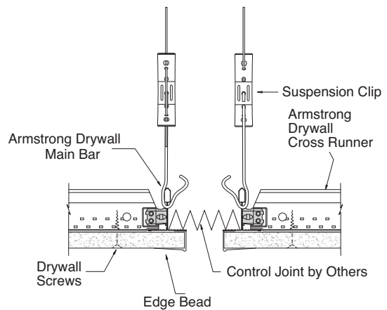
4 Control Joint
