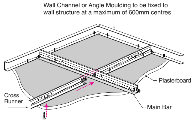
2 Perimeter Detail
