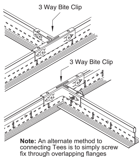
6 Securing a Single Cross Runner
